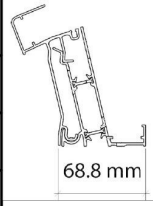
Ring beam detail
